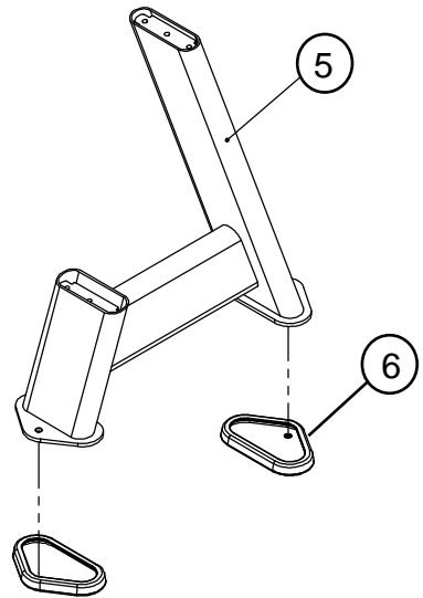
#1 P/N 52772PA-A PTD ASSY, TTDR BASE
