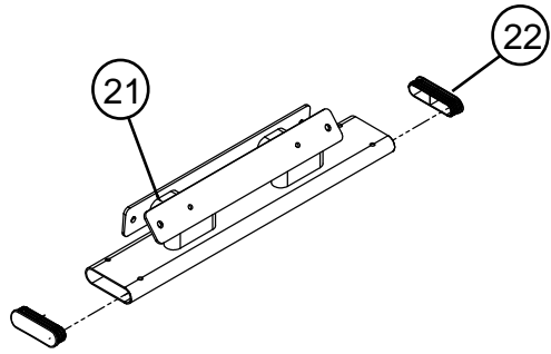
#7 P/N 53131PA-A PTD ASSY, ACB PAD SUPPORT
