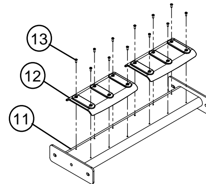
#1 P/N 53121PA-A PTD ASSY, ACB CROSS SUPPORT
