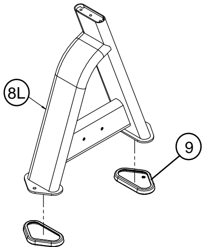
#1L P/N P20-4257 PTD ASSY, STDR BASE LEFT
