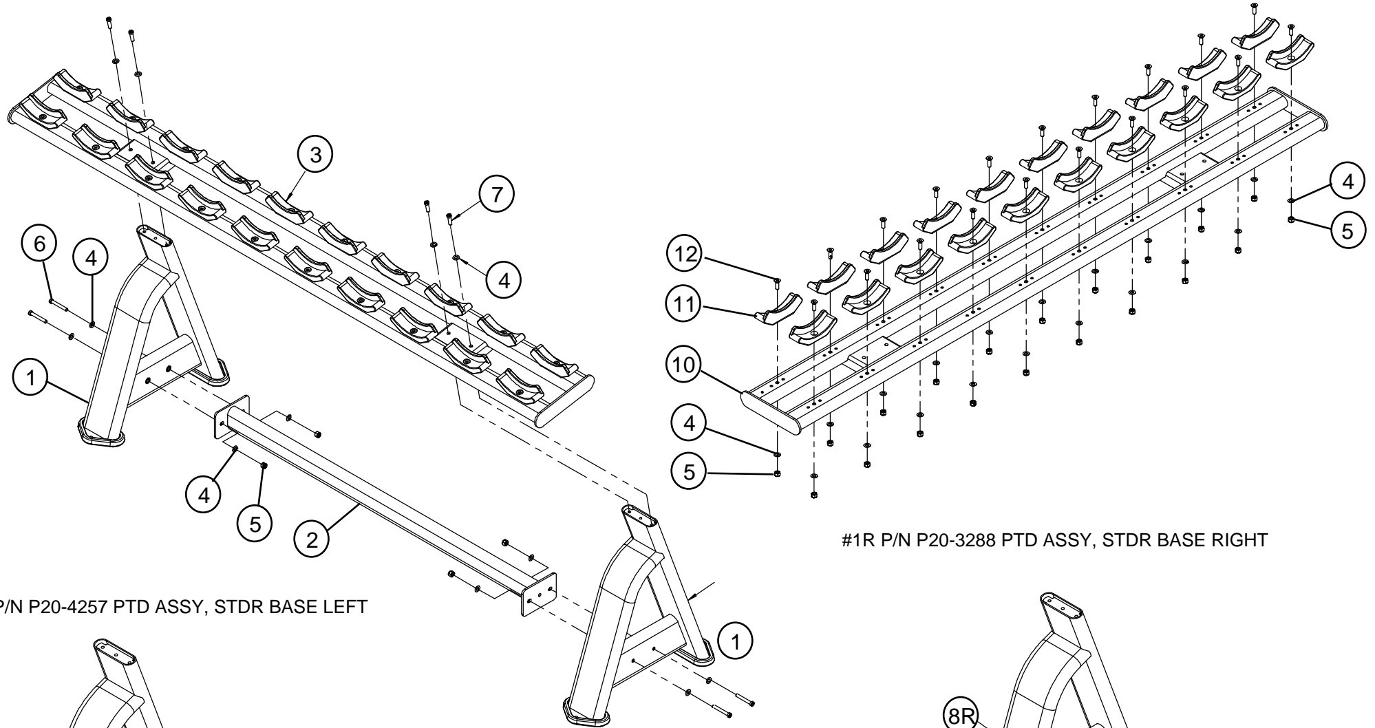
#3 P/N 52777PA PTD ASSY, RACK
